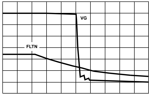
VOLTAGE (2V/DIV) TIME (10μs/DIV) FLTN = 0.1μF
